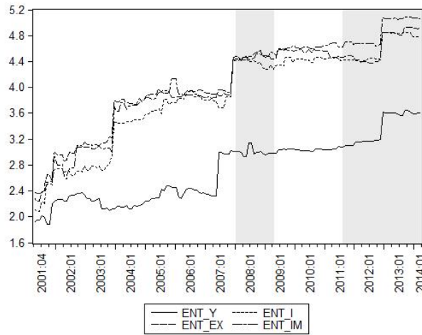
Figure 4: Entropy measures for the Euro area aggregates
