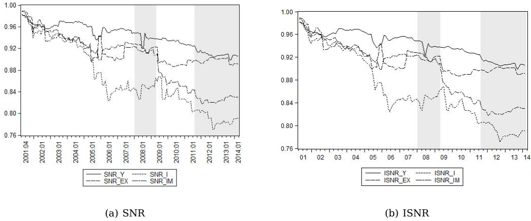
Figure 3: Signal-to-Noise Ratios for the Euro area aggregates
