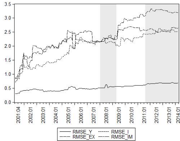
Figure 2: Root Mean Squared Errors for the Euro area aggregates
