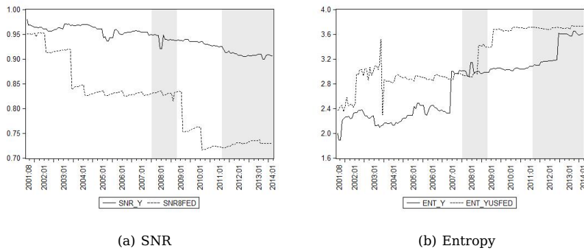
Figure 5: Comparison between the Euro area and the US real GDP uncertainty estimates
