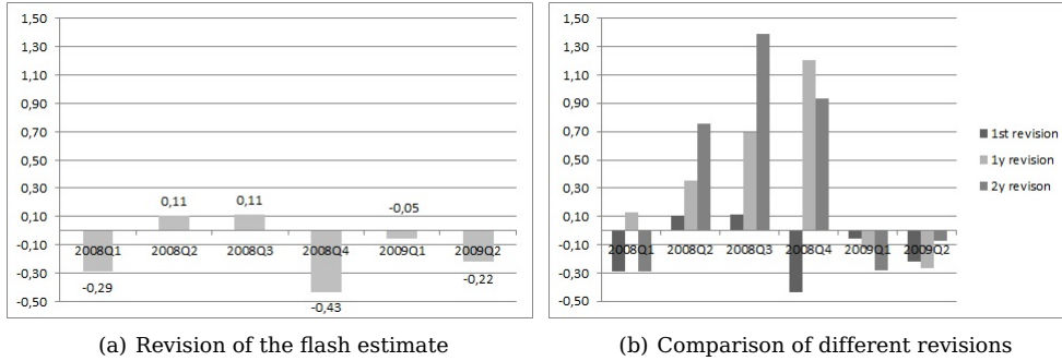
Figure 1: Revision size during the recession: Euro area real GDP growth rates
