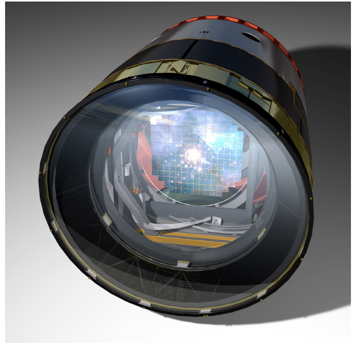
Above: SLAC is leading the construction of LSST’s 3.2-gigapixel camera, the largest digital camera ever built. (T. Mason, Mason Productions Inc./LSST Corporation) Below: Rendering of the telescope at its future site atop the Chilean mountain Cerro Pachón. (LSST Project Office)
