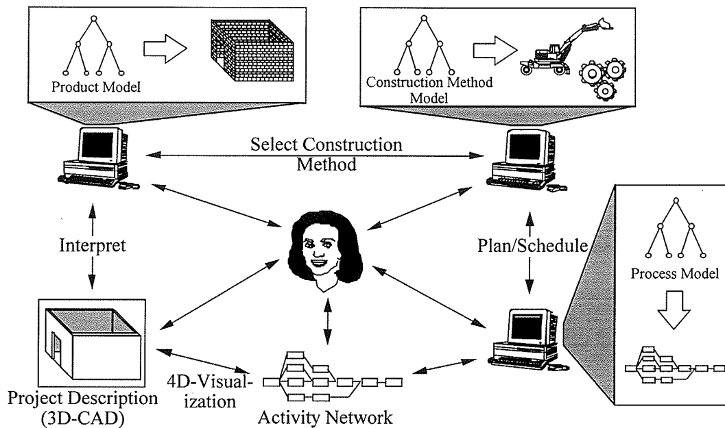
Figure 5: Symbolic and graphical facility product, construction method, and construction process models support the selection of construction methods and design of activity network alternatives. These construction management designs are done concurrently with factory design alternatives in CE4.
