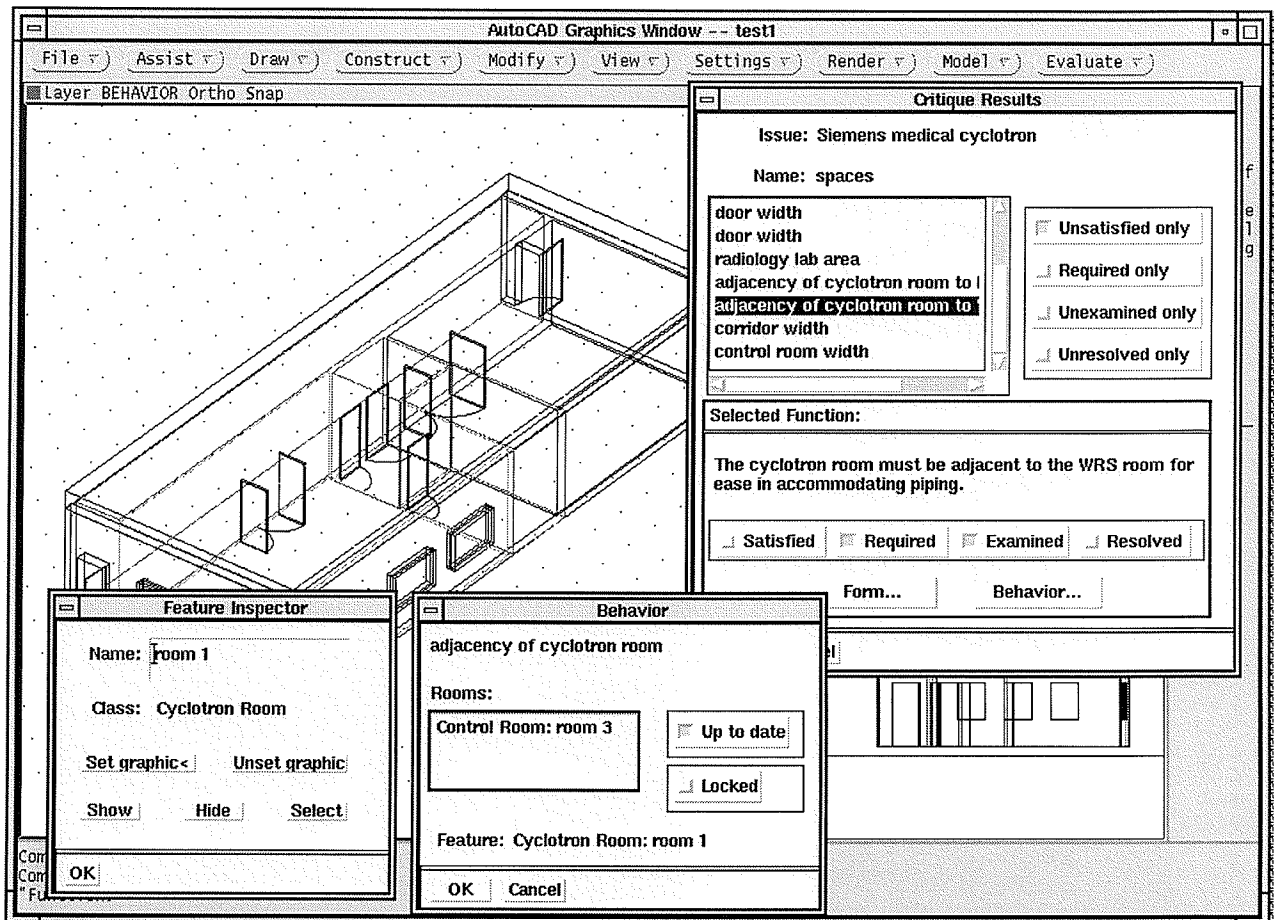
Figure 4: In the SME system concurrent design involves analysis of symbolic models of designs that normally exist, at least in part, in graphic form. SME then critiques the building design as described in the associated symbolic model. SME allows the user to define and relate both graphic and symbolic objects as needed.
