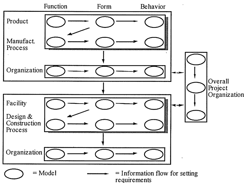
Figure 2: CE4 extends the scope of traditional concurrent engineering of product and manufacturing process (CE2) to concurrent engineering of product, process, facility and organization (CE4). CE4 also provides tools and methods to design and analyze this extended scope. The uppermost Product and Manufacturing Process rectangle shows CE2. CE4 encompasses all entities in the figure.
