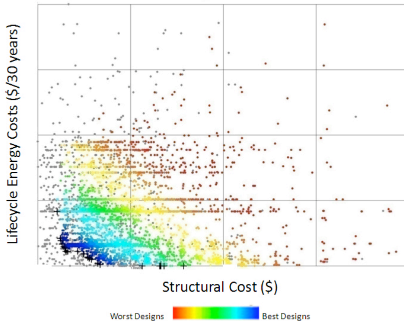
FIG. 10: Pareto front showing the trade-off between minimizing life-cycle energy costs and structural first costs
