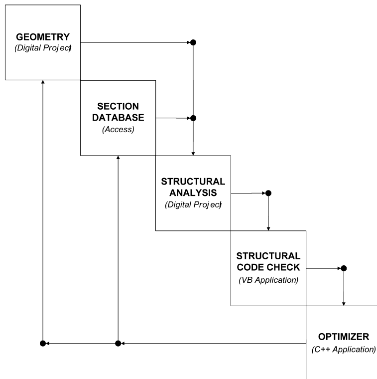
FIG. 3: Structural design, analysis, and optimization process
