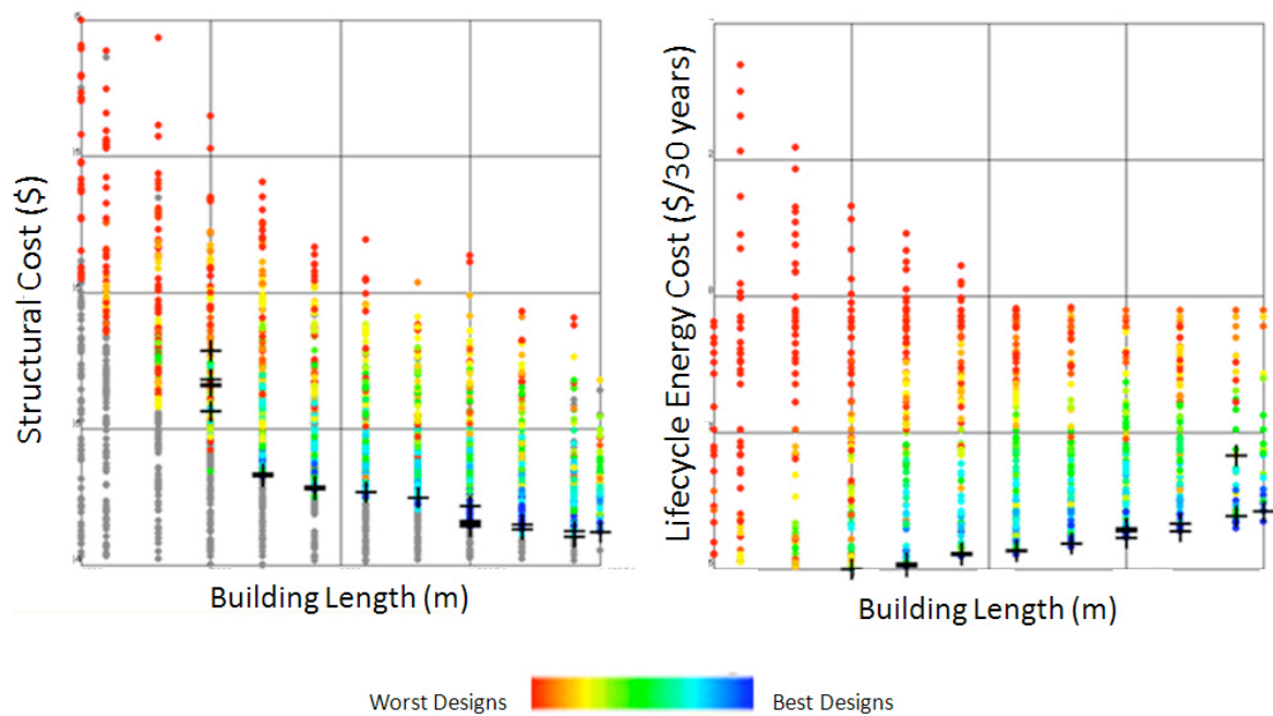
Fig. 11: When structural costs (left) and energy costs (right) are plotted against building length, the Pareto optimal designs show opposite performance trends
