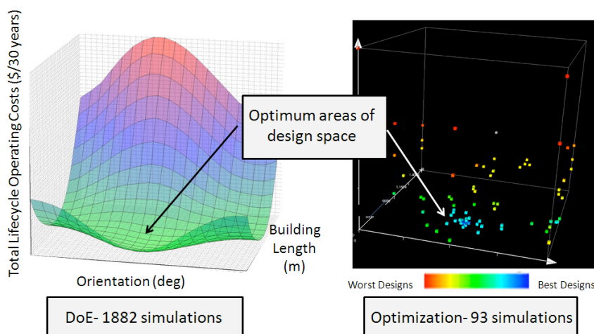
FIG. 8: DoE results vs. optimization results. Both plots show building orientation and length vs. lifecycle operating cost.
