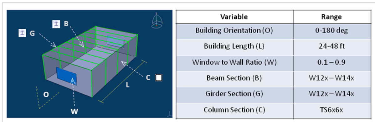
FIG. 2: Design variables for classroom case study
