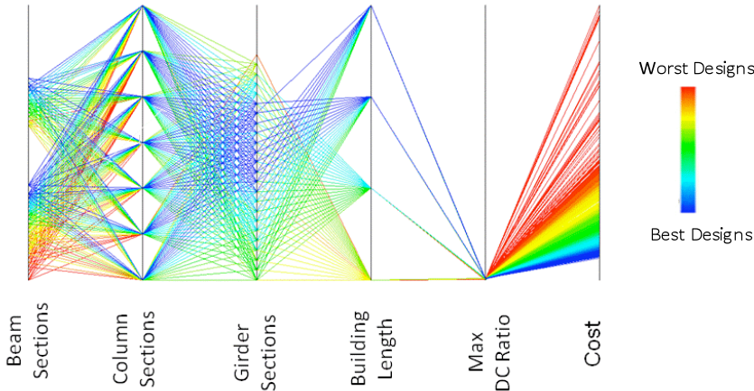
FIG. 5: Impact of structural design variables on building steel cost
