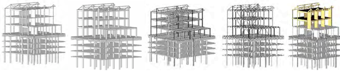
Fig. 9. Alternatives - Designers provided 3D models of typical bays for five design Alternatives (from left to right: concrete shear wall, concrete moment frame, steel braced frame, steel moment frame, and wood above concrete). The structural Alternatives were very clear.
