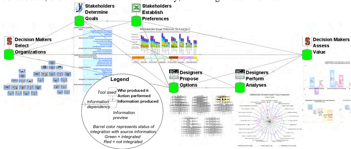
Fig. 10. MACDADI Overview – A process diagram (Haymaker, 2006) illustrating how Decision Makers, Designers, and Stakeholders interact through models of the Organizations, Objectives (Goals and Preferences), Alternatives, Analyses, and Value to assist in a systematic and transparent decision-making process.
