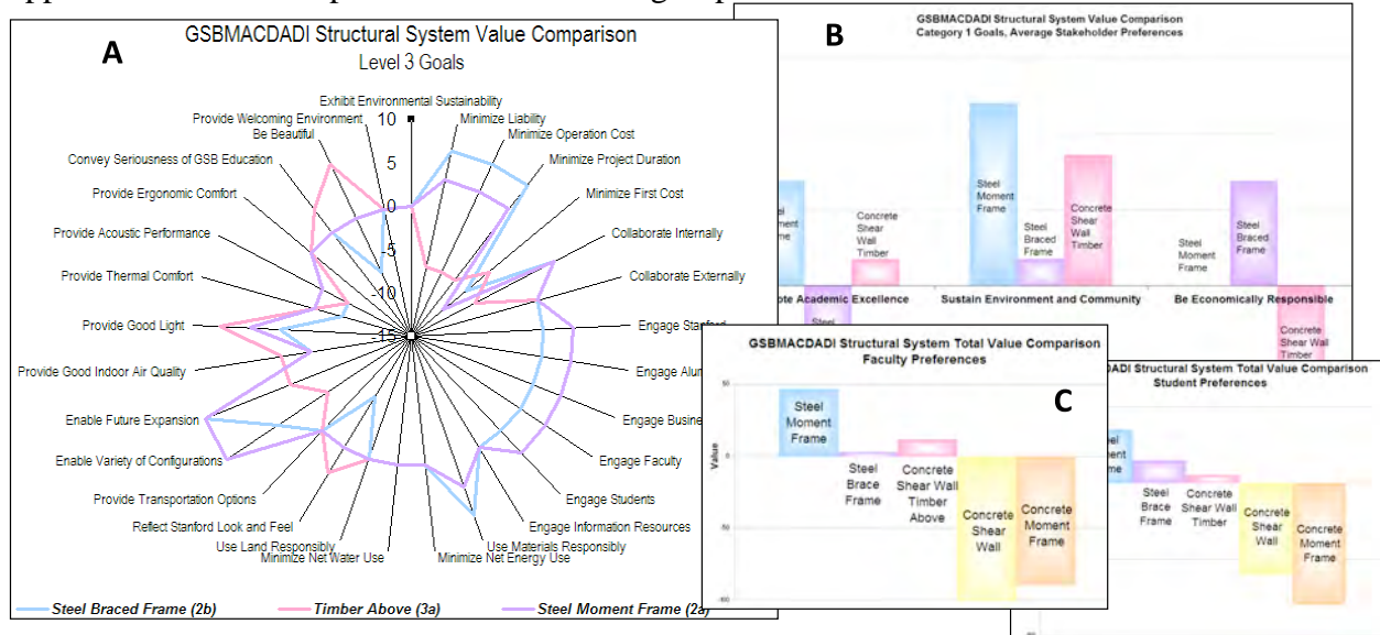
Fig. 16. Visualizing Analyses and Value: Analyses, weighted by the Stakeholder Preferences on Goals, approximate the Value of an Alternative. (A) illustrates performance Impacts of three structural Alternatives with respect to all low level Goals; (B) Value Tradeoffs of higher level Goals approximated by aggregating performance on lower level Goals; and (C) Different Stakeholder Goal Preferences are reflected in Value. While Stakeholders agree on the first choice, MACDADI illustrates that the concrete and wood Alternative provides the second highest value to the faculty, whereas the Steel Braced Frame provides the second highest value to the students.
