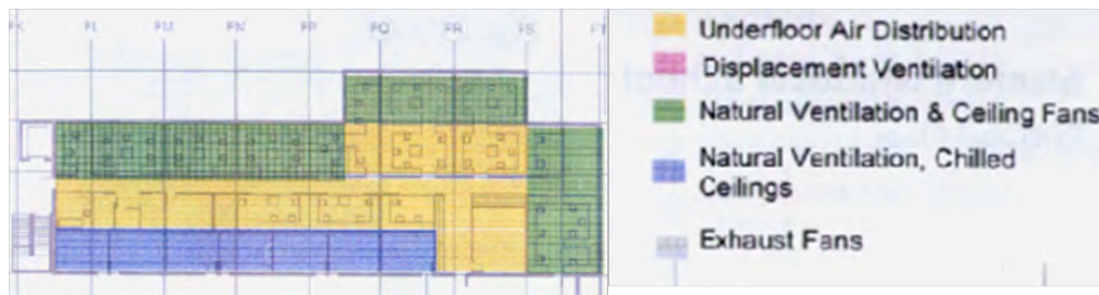
Fig. 6. A drawing by the Designers illustrates the selected mechanical system Alternative, and indicates that Management selected three different systems for the different spaces. This distinction between spaces is commonplace, but it is Inconsistent with the supporting analysis in Figure 5, which scores Alternatives without regard to location.
