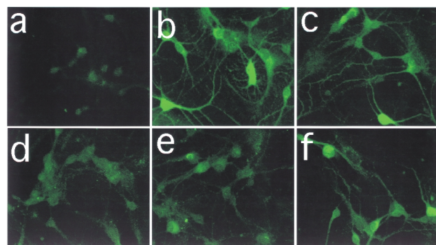
Fig. 4. Continuous upstream activation of MEK during the post-stimulus stabilized state. (a–c) Typical time course of pMAPK after four spaced depolarizing stimuli (graphed in g). (d) Effect of the MEK inhibitor U0126 (10 μM) applied after stimulation, showing the same prompt reduction of pMAPK as found with PD98059. Removal of this MEK inhibitor allowed a prompt return of pMAPK from baseline to its stabilized level (e, f), pointing to a continuous upstream activation of MEK.
