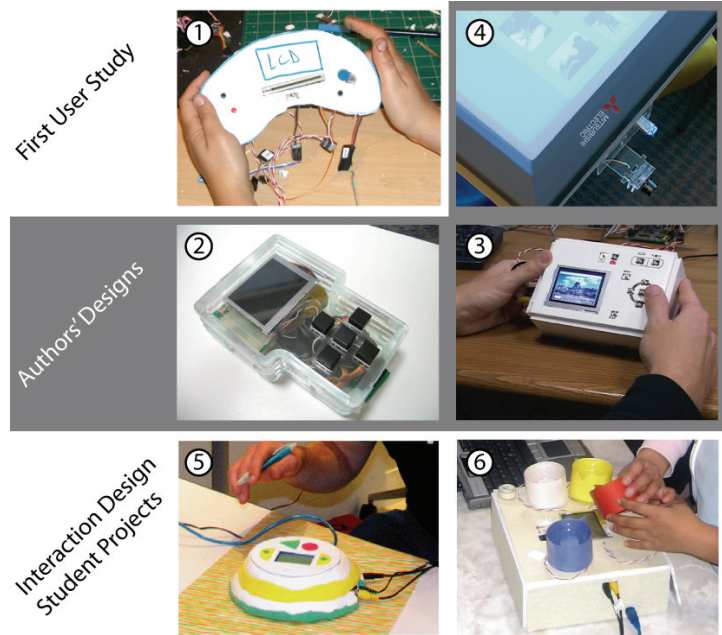
Figure 7 A selection of projects built with d.tools. (1) music player for children; (2) media player; (3) digital camera back; (4) tangible drawer for a tabletop display; (5) voice message trading pebble; (6) tangible color mixer.
