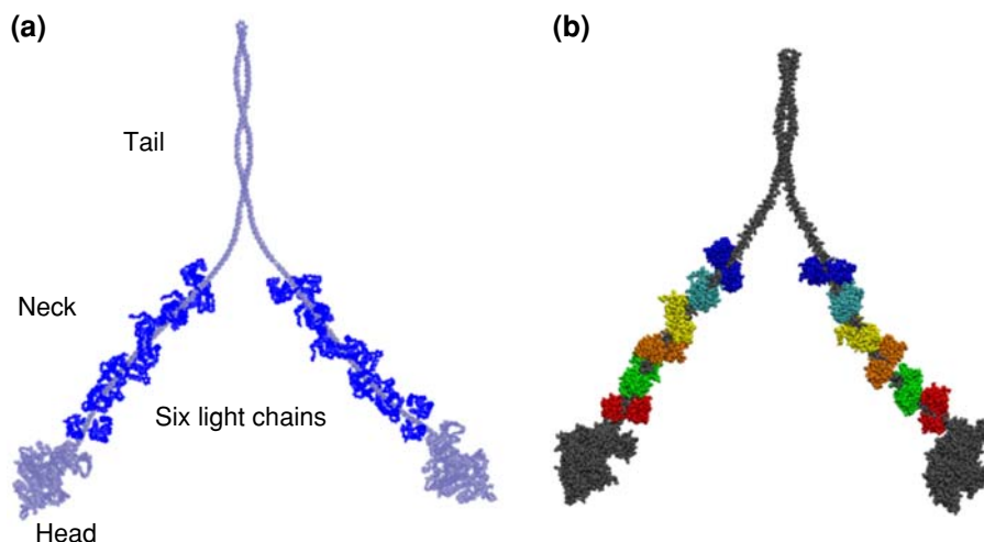
FIGURE 3. Structure and coarse-grained model of the myosin V molecule. (a) A myosin V molecule (gray) consists of head, neck, and tail regions. The head region binds actin and hydrolyzes ATP. Extending from the head is the neck region, a long \alpha -helix containing six IQ motifs, each of which binds a single calmodulin-like light chain (blue). The \alpha -helices of two myosin V molecules dimerize to form a coiled-coil tail region. (b) Atomic resolution model of the myosin V dimer.
