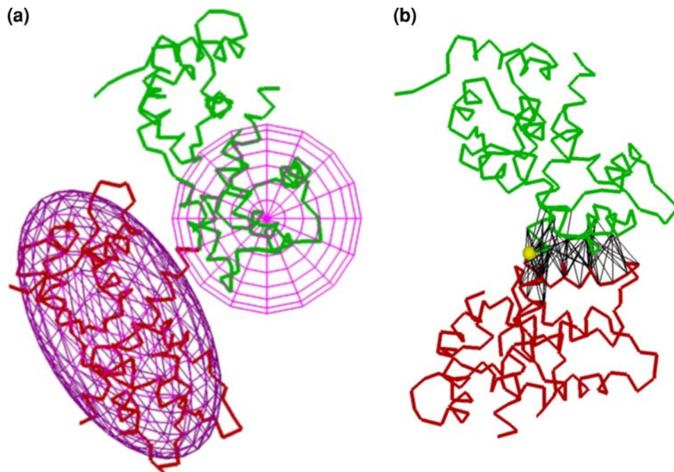
FIGURE 2. Modeling physical interactions. (a) Contact potential geometry for two rigid domains (colored red and green), each comprising a calmodulin molecule bound to a myosin V IQ motif helix (colored red and green). An ellipsoid has been defined for the entire lower domain while a sphere has been defined for a portion of the upper domain (colored purple). (b) A spring potential defined for two rigid domains. C_{\alpha} atoms between the two domains within 8 Å of each other are connected by harmonic springs shown as black lines.
