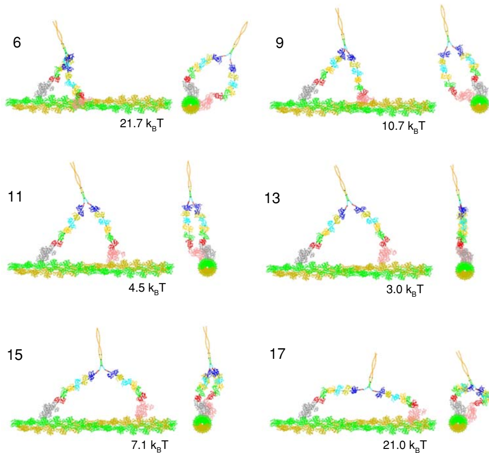
FIGURE 5. Conformations of a myosin V dimer spanning different numbers of actin binding sites. The leading head (colored pink) is bound 6, 9, 11, 13, 15, or 17 actin subunits from the bound rear head (colored gray). The elastic strain energy for each conformation is shown below the actin filament.
