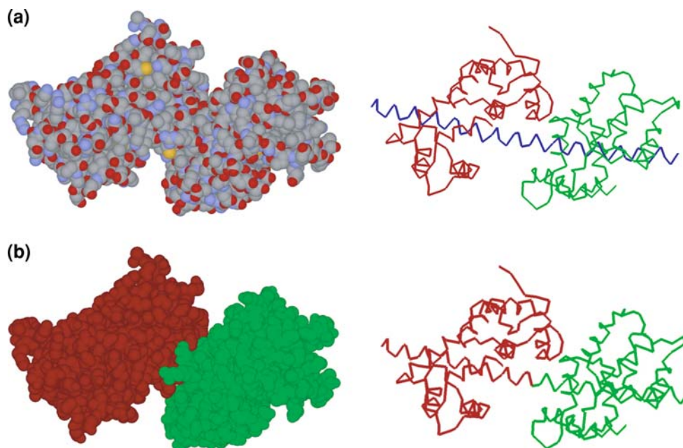
FIGURE 1. Domain definition and molecular representations in the Protein Mechanics software. (a) Visualization of the atomic structure of two calmodulin molecules bound to the central \alpha -helix. In the space-filling representation ( left ), atoms are colored by atom type. In the C_\alpha backbone trace representation ( right ), the calmodulin chains are colored red and green, and the helix is blue. (b) Two domains ( colored red and green ) defined to each comprise a portion of the \alpha -helix together with its bound calmodulin. The domains are shown using space-filling atoms ( left ) and C_\alpha backbone ( right ) representations.
