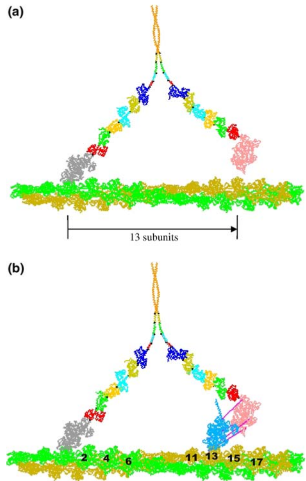
FIGURE 4. Coarse-grained model of a myosin V dimer. (a) Each myosin monomer has been substructured into 12 rigid bodies (shown using a C_\alpha backbone representation and different colors for each domain) connected by ball joints (shown as black spheres ). The rear and leading heads are in a post-powerstroke and pre-powerstroke conformation, respectively. The rear head ( colored gray ) is bound to an actin filament ( colored green and yellow ) while the leading head ( colored pink ) is free. (b) Restraints ( colored purple ) defined between the free head and a “ghost” actin-bound reference head ( colored blue ) will pull the free head and align it to the desired binding site during a simulation. Actin subunits are numbered on the actin filament relative to the binding site of the trailing head.
