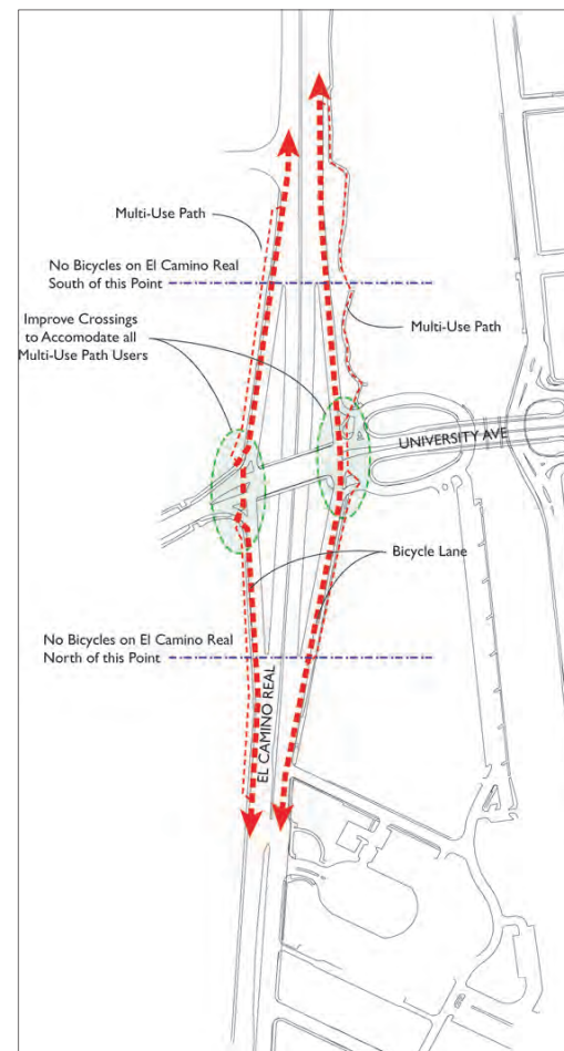
Figure 5.32: A multi-use path above ground which crosses University Avenue can be added as part of the intersection redesign called for in the PAITC.
