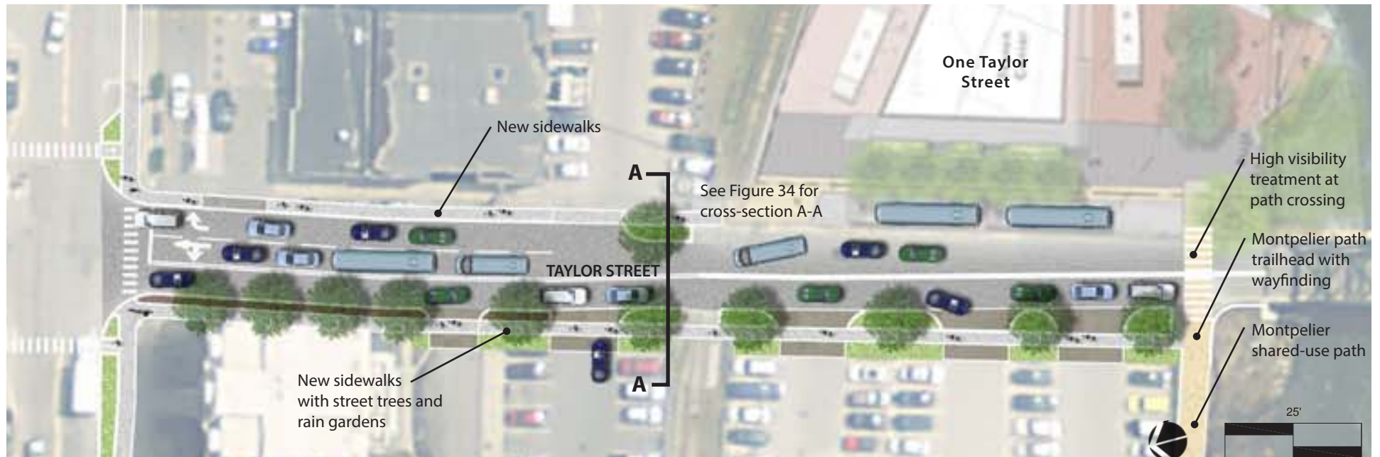
Figure 35: Design option for Taylor Street.
