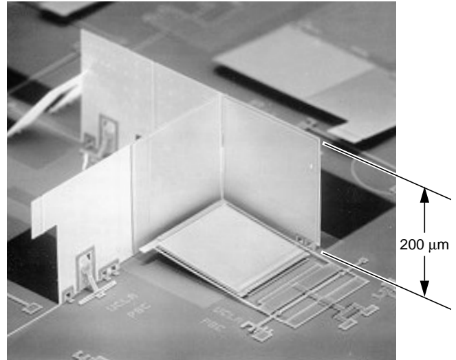
Figure 2. Microfabricated corner-cube retroreflector, consisting of three gold-coated polysilicon mirrors. The base mirror can be deflected electrostatically, modulating the optical signal reflected from the device (taken from [2]).
