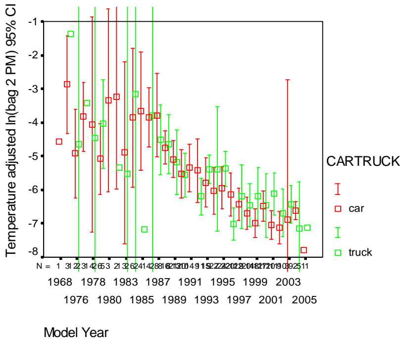
Figure 33. Temperature adjusted natural log of hot running PM as a function of model year bin.
