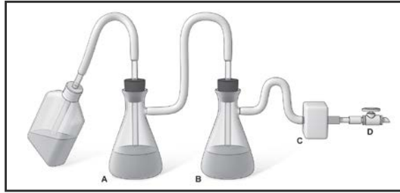
Figure 1. Liquid Waste. The left suction flask (A) is used to collect the contaminated fluids into a suitable decontamination solution; the right flask (B) serves as a fluid overflow collection vessel. An in-line HEPA filter (C) is used to protect the vacuum system (D) from microorganisms.
