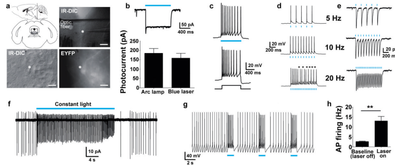
Figure 5. Functional characterization of TPH2-ChR2(H134R)-EYFP BAC transgenic mice. (a) Diagram of acute coronal brainstem slice preparation and representative image showing placement of the optic fiber in the region of a recorded neuron (top). Scale bar: 200 \mu\text{m} . IR-DIC and EYFP fluorescence image of a recorded 5-HT neuron in the dorsal raphe nucleus (bottom). Scale bar: 20 \mu\text{m} . (b) Voltage clamp recording of a 5-HT neuron demonstrating inward current induced by blue laser light ( 26.3 \text{ mW mm}^{-2} ) (top). Plot of peak steady-state photocurrent in response to blue light delivered as indicated (bottom). (c) Current clamp mode recording showing action potential firing in response to blue laser light ( 26.3 \text{ mW mm}^{-2} ) (top) or in response to +100 pA current injection (bottom). (d–e) Current clamp mode (d) and voltage clamp (e) recording of responses to patterned blue laser light ( 26.3 \text{ mW mm}^{-2} , 5 ms pulse width). Asterisks indicate missed action potentials. Note: in panels c–d a small hyperpolarizing current injection was applied to silence basal firing. (f, g) Cell-attached recording of a 5-HT neuron under prolonged constant blue light stimulation (f) or to repeated bouts of blue light (g). (h) Summary plot of baseline and blue light-induced firing rates. ** P < 0.01 (one-tailed paired t-test).
