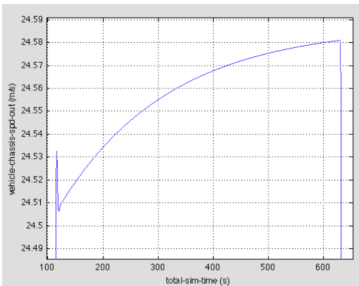
Figure 3 - Actual vehicle chassis speed during the constant speed demand portion of the 55 mph drive cycle.
