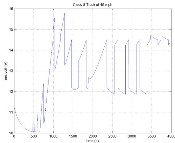
Figure 1: Irregular Voltage of Battery
