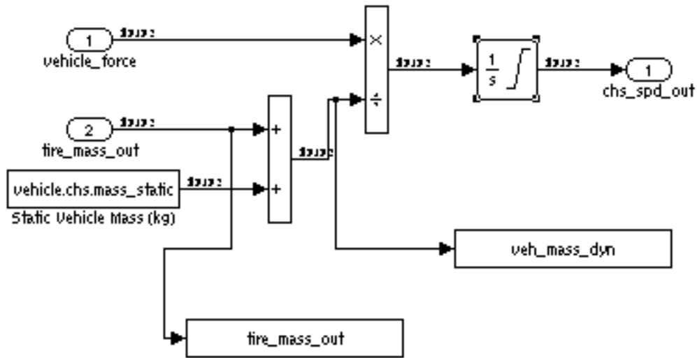
Figure 1 - Section of the GEM Simulink model where vehicle speed is calculated.
