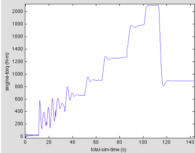
Figure 4 - Engine torque during acceleration ramp in 55 mph drive cycle.
