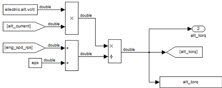
Figure 2: Possible Error in Alternator Mechanical Torque Calculation
