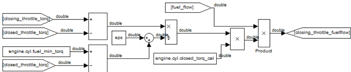
Figure 5: Closed-Throttle Fuel Flow Calculation
