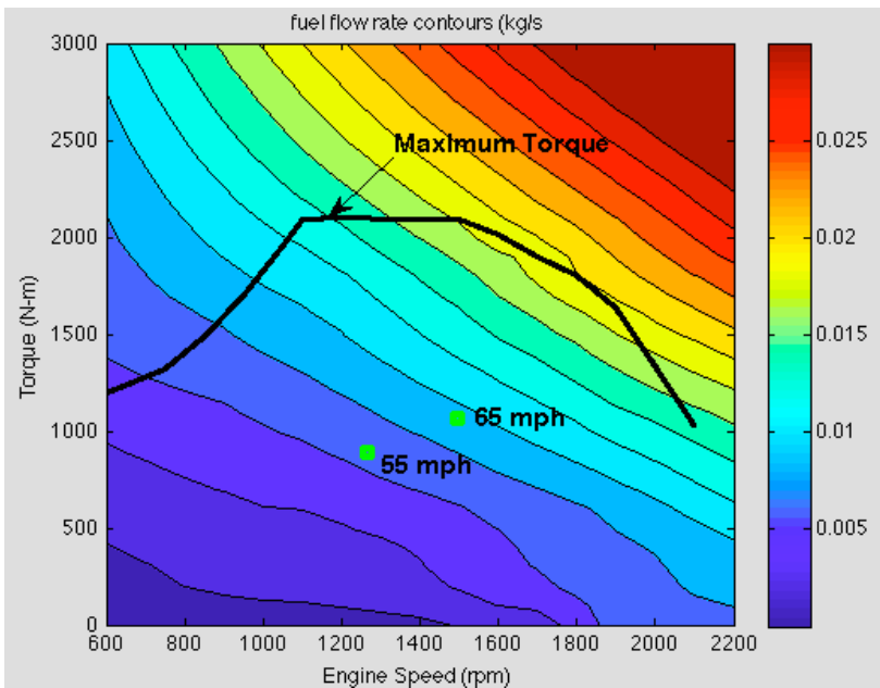
Figure 5 - contours of fuel flow rate versus engine speed and torque for 15L engine from "engine_map_455.m".
