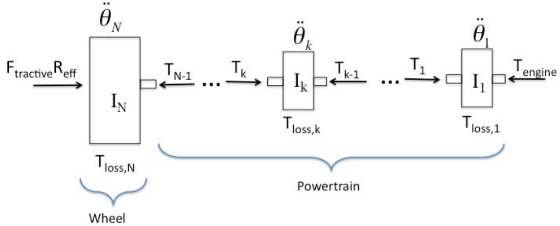
Figure a7 - Torque transfer from the engine, through the powertrain, to the tires.
