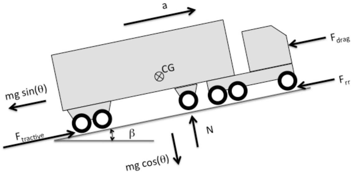
Figure a6 - Free body diagram showing forces and accelerations on a vehicle
