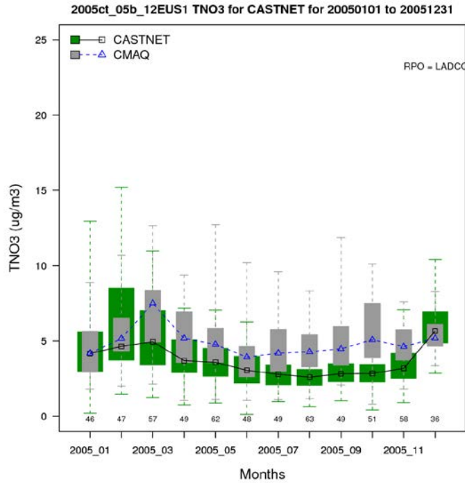
Figure A-23c. Distribution of observed and predicted weekly average total nitrate by month for 2005 at CASTNet sites in the Midwest subregion.
