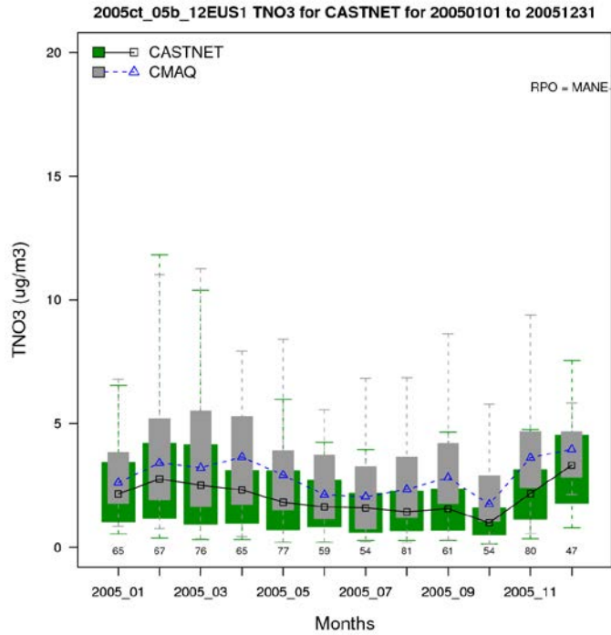
Figure A-21c. Distribution of observed and predicted weekly average total nitrate by month for 2005 at CASTNet sites in the Northeast subregion.
