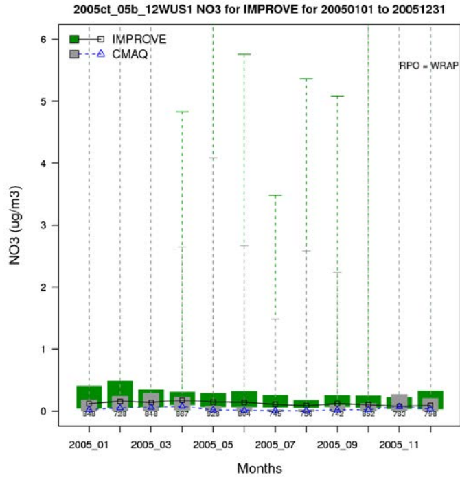
Figure A-25a. Distribution of observed and predicted 24-hour average nitrate by month for 2005 at IMPROVE sites in the Western states subregion.
