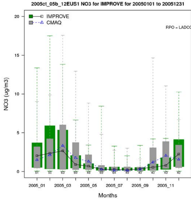
Figure A-23a. Distribution of observed and predicted 24-hour average nitrate by month for 2005 at IMPROVE sites in the Midwest subregion.
