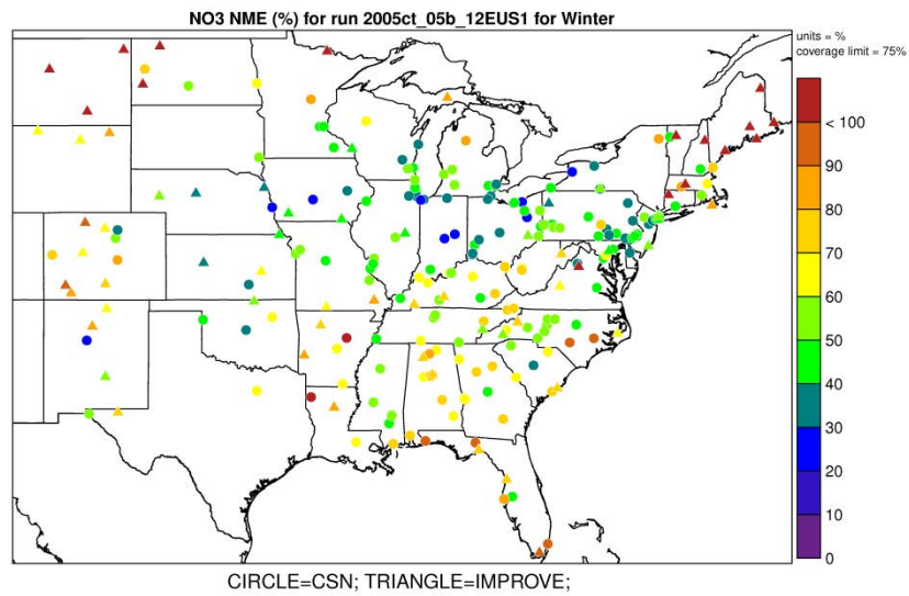
Figure A-26b. Normalized Mean Error (%) for nitrate during winter 2005 at monitoring sites in Eastern modeling domain.
