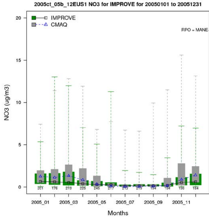
Figure A-21a. Distribution of observed and predicted 24-hour average nitrate by month for 2005 at IMPROVE sites in the Northeast subregion. [symbol = median; top/bottom of box = 75 th /25 th percentiles; top/bottom line = max/min values]
