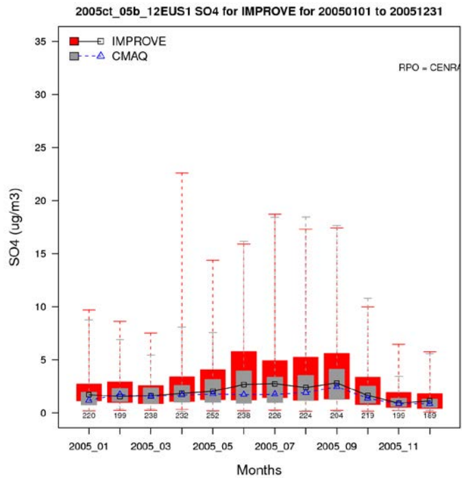
Figure A-11a. Distribution of observed and predicted 24-hour average sulfate by month for 2005 at IMPROVE sites in the Central states subregion.
