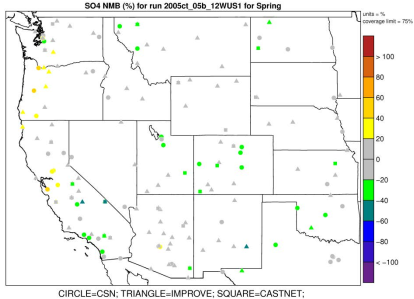
Figure A-18a. Normalized Mean Bias (%) of sulfate during spring 2005 at monitoring sites in Western modeling domain.
