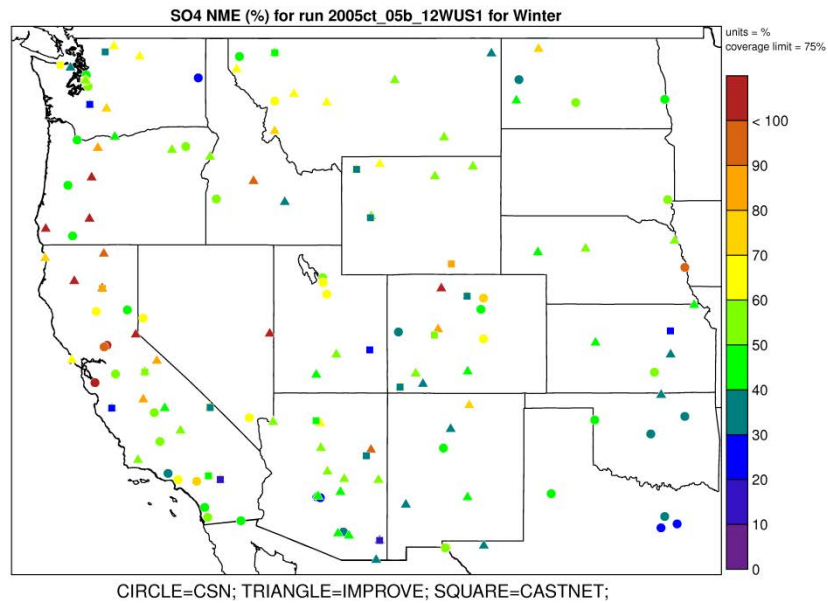
Figure F-17b. Normalized Mean Error (%) of sulfate during winter 2005 at monitoring sites in Western modeling domain.
