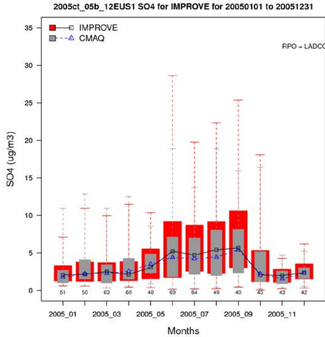
Figure A-10a. Distribution of observed and predicted 24-hour average sulfate by month for 2005 at IMPROVE sites in the Midwest subregion.
