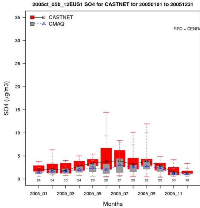
Figure A-11c. Distribution of observed and predicted weekly average sulfate by month for 2005 at CASTNet sites in the Central states subregion.
