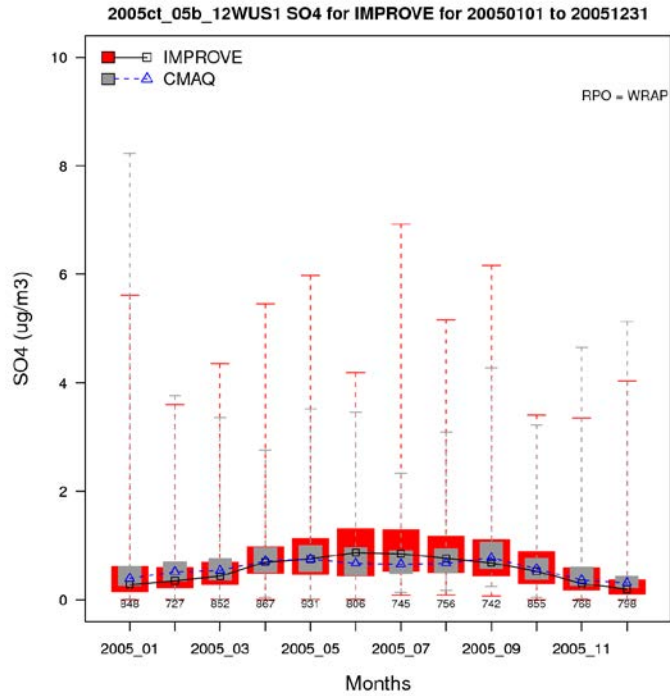
Figure A-12a. Distribution of observed and predicted 24-hour average sulfate by month for 2005 at IMPROVE sites in the Western states subregion.
