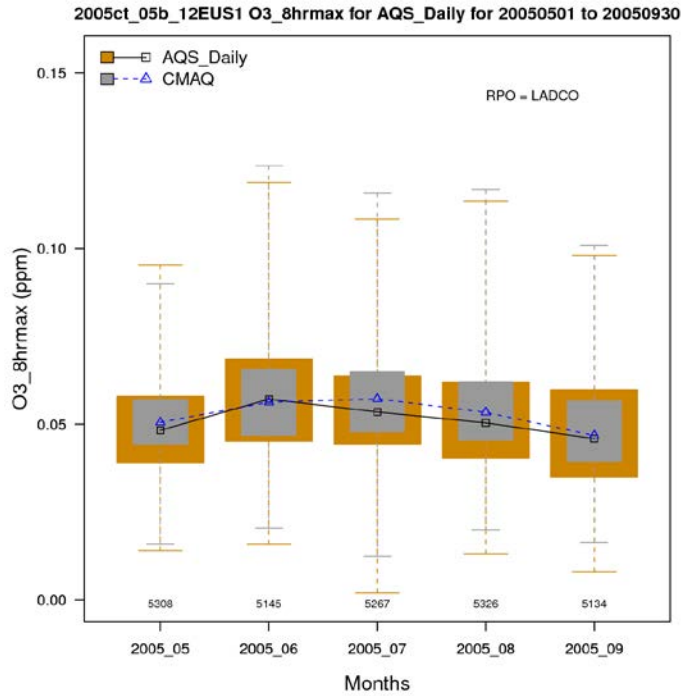
Figure A-3. Distribution of observed and predicted 8-hour daily maximum ozone by month for the period May through September for the Midwest subregion.
