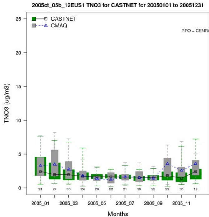
Figure A-24c. Distribution of observed and predicted weekly average total nitrate by month for 2005 at CASTNET sites in the Central states subregion.
