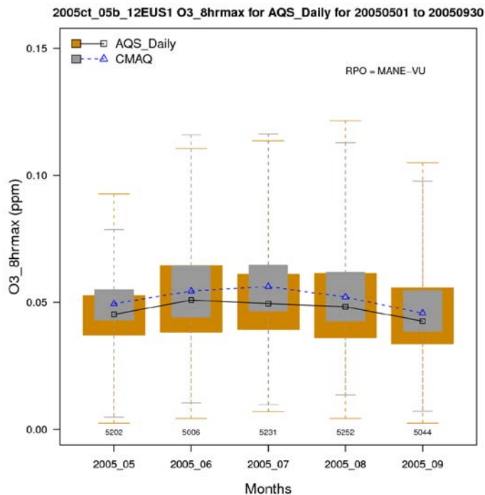
Figure A-1. Distribution of observed and predicted 8-hour daily maximum ozone by month for the period May through September for the Northeast subregion. [symbol = median; top/bottom of box = 75 th /25 th percentiles; top/bottom line = max/min values]
