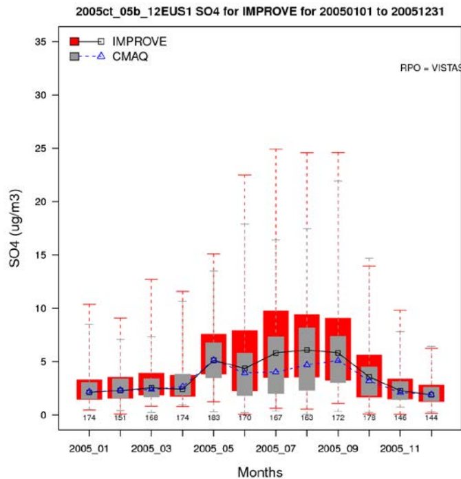
Figure A-9a. Distribution of observed and predicted 24-hour average sulfate by month for 2005 at IMPROVE sites in the Southeast subregion.
