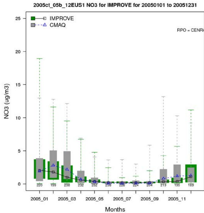
Figure A-24a. Distribution of observed and predicted 24-hour average nitrate by month for 2005 at IMPROVE sites in the Central states subregion.
