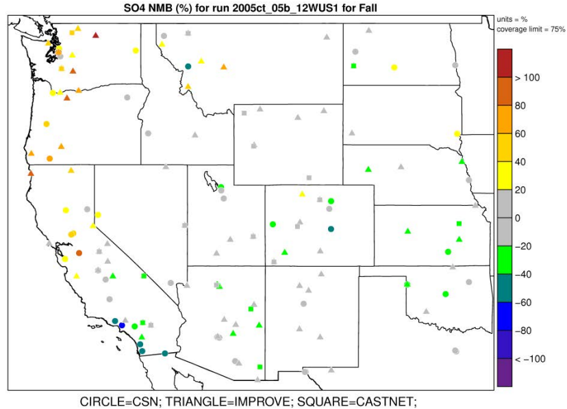
Figure A-20a. Normalized Mean Bias (%) of sulfate during fall 2005 at monitoring sites in Western modeling domain.
