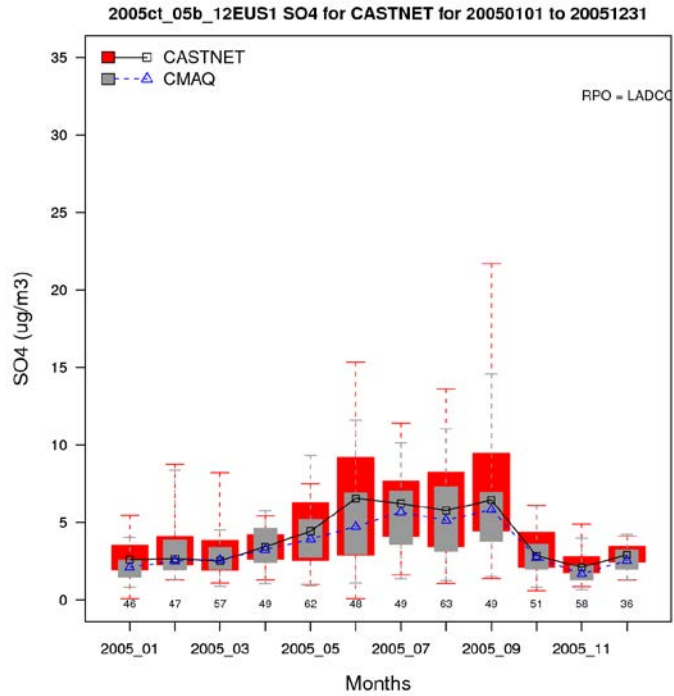
Figure A-10c. Distribution of observed and predicted weekly average sulfate by month for 2005 at CASTNet sites in the Midwest subregion.
