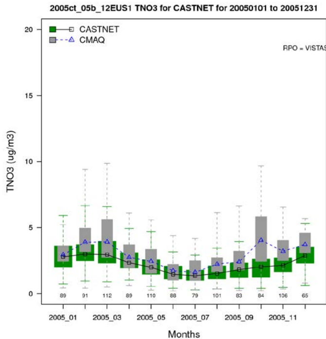
Figure A-22c. Distribution of observed and predicted weekly average total nitrate by month for 2005 at CASTNET sites in the Southeast subregion.
