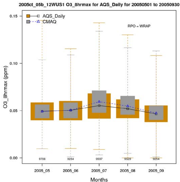
Figure A-5. Distribution of observed and predicted 8-hour daily maximum ozone by month for the period May through September for the Western states subregion.
