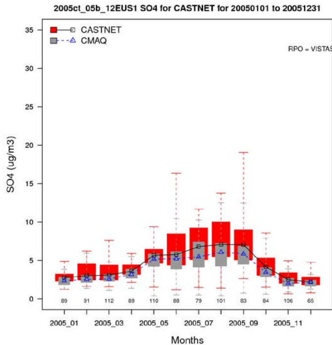
Figure A-9c. Distribution of observed and predicted weekly average sulfate by month for 2005 at CASTNet sites in the Southeast subregion.
