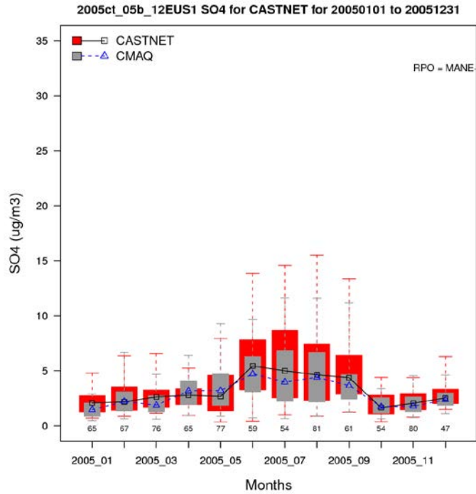
Figure A-8c. Distribution of observed and predicted weekly average sulfate by month for 2005 at CASTNet sites in the Northeast subregion.
