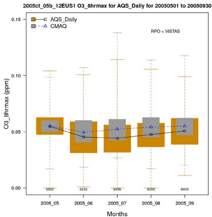
Figure A-2. Distribution of observed and predicted 8-hour daily maximum ozone by month for the period May through September 2005 for the Southeast subregion.
