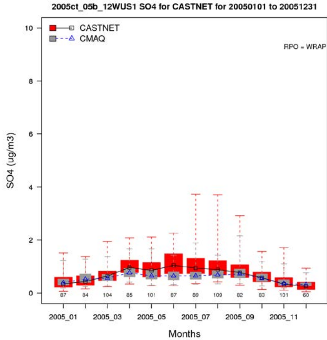
Figure A-12c. Distribution of observed and predicted weekly average sulfate by month for 2005 at CASTNet sites in the Western states subregion.
