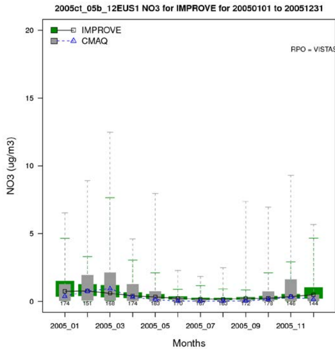
Figure A-22a. Distribution of observed and predicted 24-hour average nitrate by month for 2005 at IMPROVE sites in the Southeast subregion.
