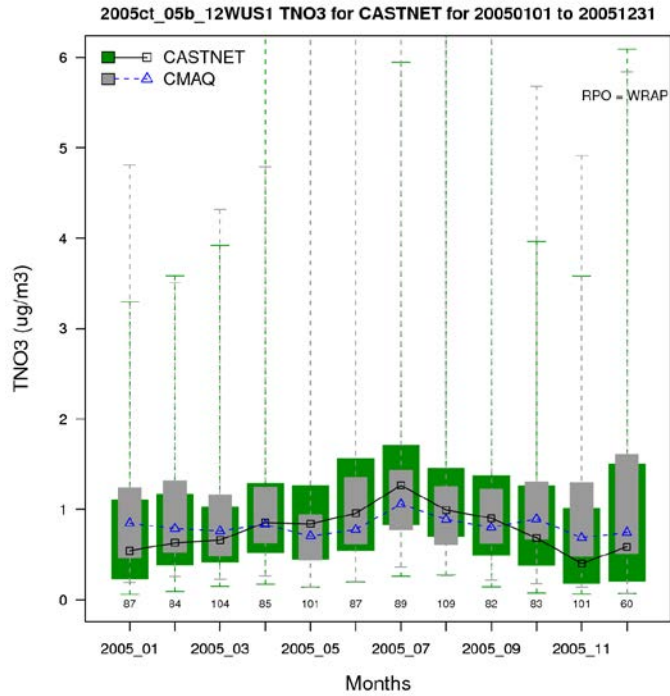
Figure A-25c. Distribution of observed and predicted weekly average total nitrate by month for 2005 at CASTNet sites in the Western states subregion.
