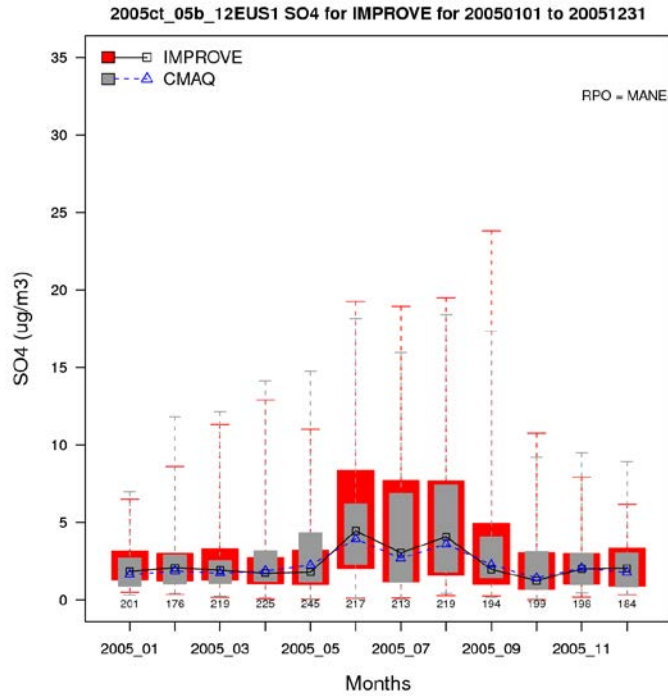
Figure A-8a. Distribution of observed and predicted 24-hour average sulfate by month for 2005 at IMPROVE sites in the Northeast subregion. [symbol = median; top/bottom of box = 75 th /25 th percentiles; top/bottom line = max/min values]
