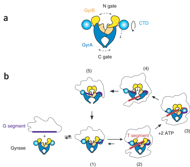
Figure 1 Gyrase subunit composition and mechanism of action. (a) Gyrase is a heterotetramer composed of two monomers of GyrA (blue) and two of GyrB (yellow). The N-terminal domains of GyrA (dark blue) interact with DNA and GyrB and form the DNA exit, or C gate. The C-terminal domains of GyrA (GyrA-CTDs, blue spheres) fold independently and are linked to the N-terminal domain of GyrA by a flexible linker, which gives them rotational and translational flexibility 47 (arrows). GyrA-CTDs are responsible for DNA binding and wrapping. GyrB interacts with DNA and GyrA, is responsible for ATP binding and hydrolysis, and forms the DNA entrance, or N gate. (b) Model for introduction of (–) supercoiling by gyrase. A gyrase complex binds a DNA fragment, called the G segment (1). From this state, there is a force-dependent kinetic competition between DNA wrapping and dissociation. After wrapping (2) and ATP binding (3), the enzyme can proceed with the strand-passage reaction (4), which leads it to a state (5) that can be reset to commence a new catalytic cycle.
