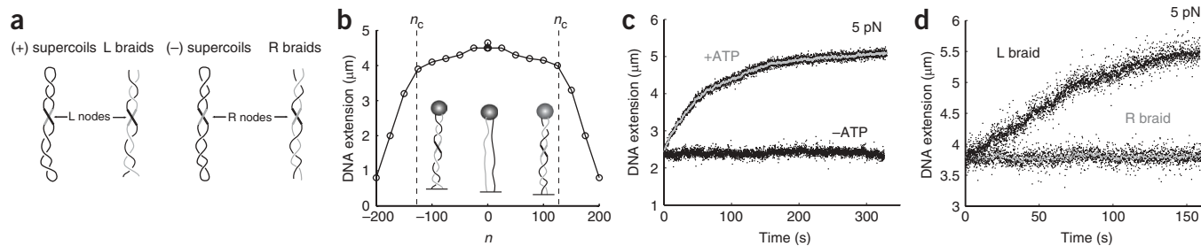
Figure 6 Gyrase unbraids DNA. (a) DNA crossings in plectonemic and braided DNA. In (+) supercoiled DNA, the crossings are left-handed (L crossings), as in left-handed braids (L braids). In contrast, DNA crossings are right handed (R crossings) on (-) supercoiled DNA and right-handed braids (R braids). (b) Variation of the extension of DNA with the number of turns n introduced for a tether with two nicked DNA molecules under constant tension. Introduction of (-) turns by rotation of the magnets leads to the formation of first-order L braids, whereas the introduction of (+) turns produces first-order R braids. As in the case of a single topologically constrained DNA molecule, beyond a critical number of turns ( n > n_c ), the DNA braids buckle to form second-order DNA braids (supercoils of braids). (c) Gyrase relaxes L braids only in the presence of ATP. Gyrase activity was followed by monitoring the braid extension at constant tension (5 pN). Only in the presence of 1 mM ATP was gyrase able to relax an L braid ( \sigma_{br} = -0.2 ; black curve, no ATP; gray curve, 1 mM ATP). Raw data are plotted in black and 1-s moving averages are shown as solid curves. (d) Preferential relaxation of L braids (5 pN). In the presence of 1 mM ATP, gyrase was able to relax first-order L braids ( \sigma_{br} = -0.07 , black curve) but not first-order R braids ( \sigma_{br} = +0.07 , gray curve). The mean unbraiding rate was \sim 10 \pm 3 \text{ nm s}^{-1} . Raw data are plotted in black and 1-s moving averages are shown as solid curves.
