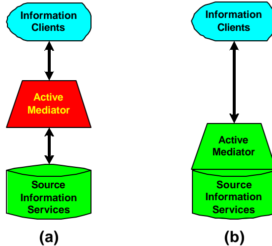
Figure 5: Incorporation of Active Mediation with Information Services
