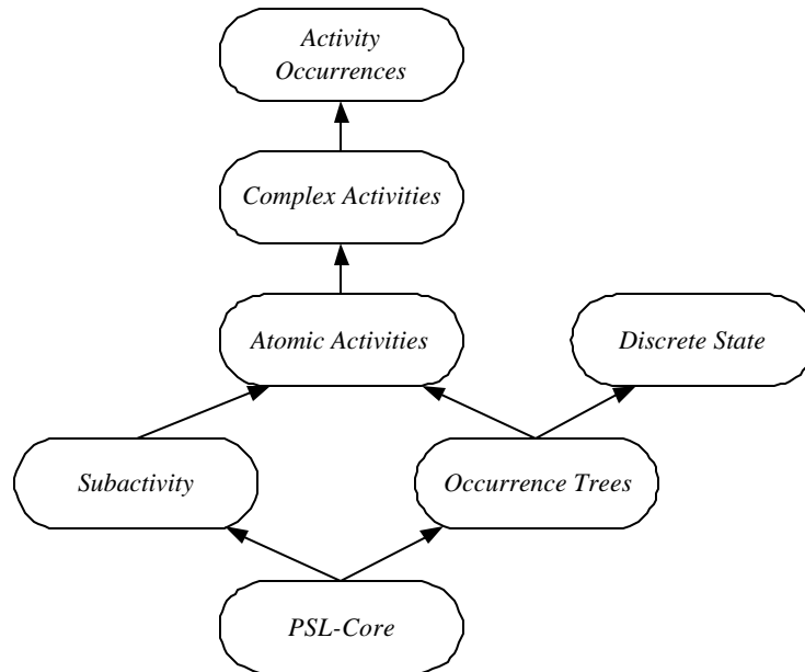
Figure 7: PSL Ontology
