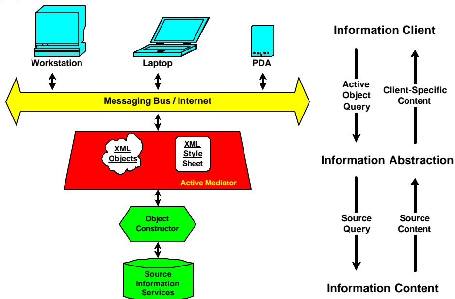
Figure 6: Active Mediation in Information Service Construction
