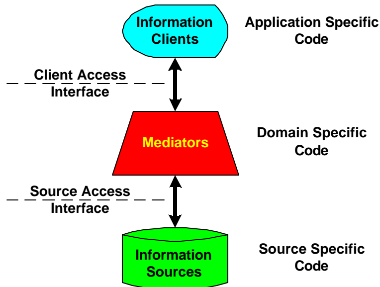
Figure 1: Mediation Architecture
