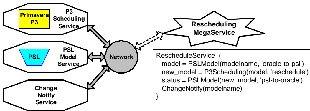
Figure 12: Rescheduling Megaservice
