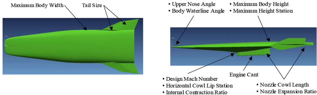
figure 5: Design variables selected for vehicle optimization 2
