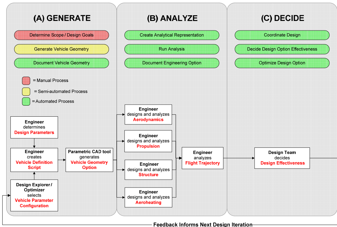
Figure 4: A systematic design space exploration process for aerospace vehicle design [based on Vandenbrande et. al. 2006, Fig.7]
