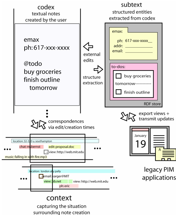
Figure 5. Architecture of Jourknow, illustrating how components of the data model (codex, subtext, and context) interact.
