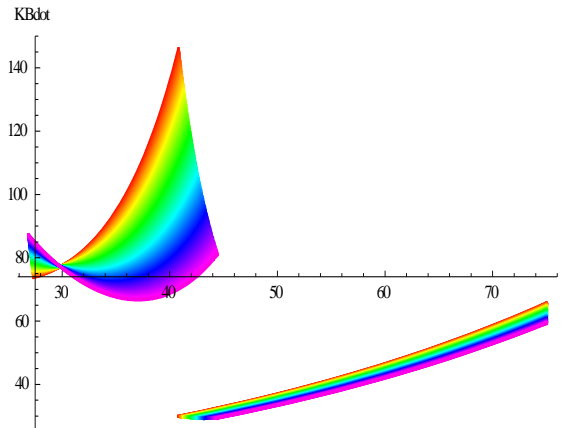
Figure 5.6.C \dot{K}_B : \delta_A^H = 0.0375 - 0.075
