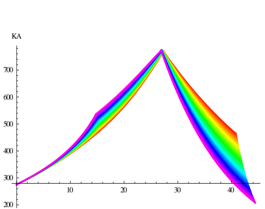
Figure 5.6.B K_A : \delta_A^H = 0.0375 - 0.075
