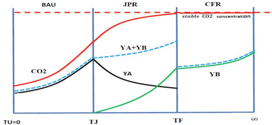
Figure 4. The 3 - Phase “Basic” (Technology Switching) Model:
