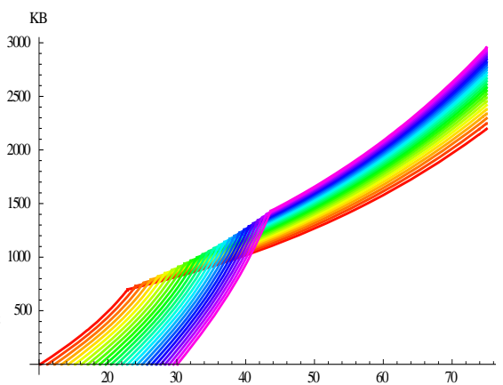
Figure 5.2.D K_B : Emax=125-375
