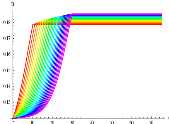
Figure 5.1 Time paths of capital productivity B
