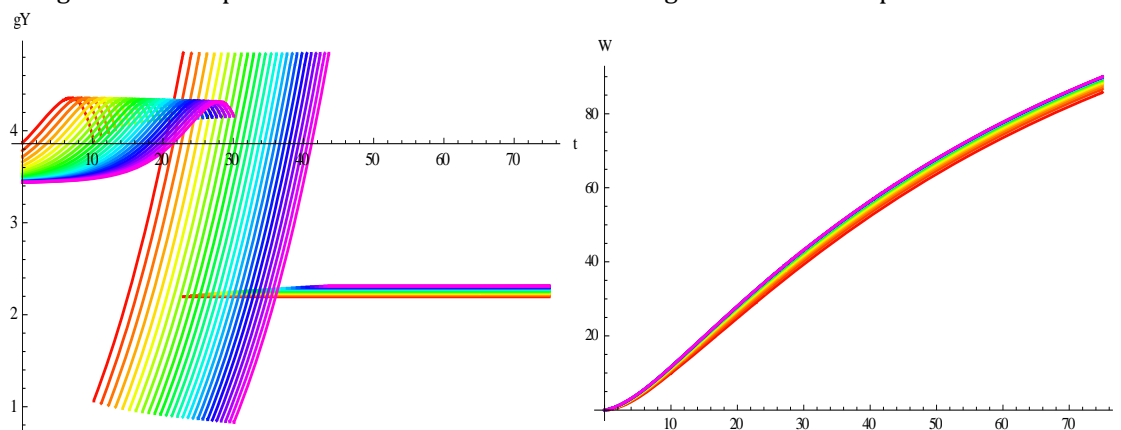
Figure 5.2.H Growth rate \dot{Y}/Y : Emax=125-375
