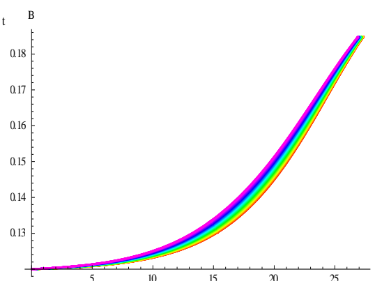
Figure 5.5 Carbon-free capital productivity, B
