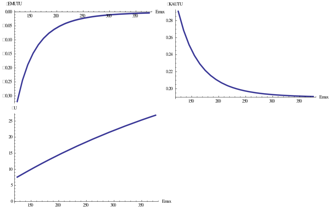
Figure 2.3 Sensitivity results BAM
