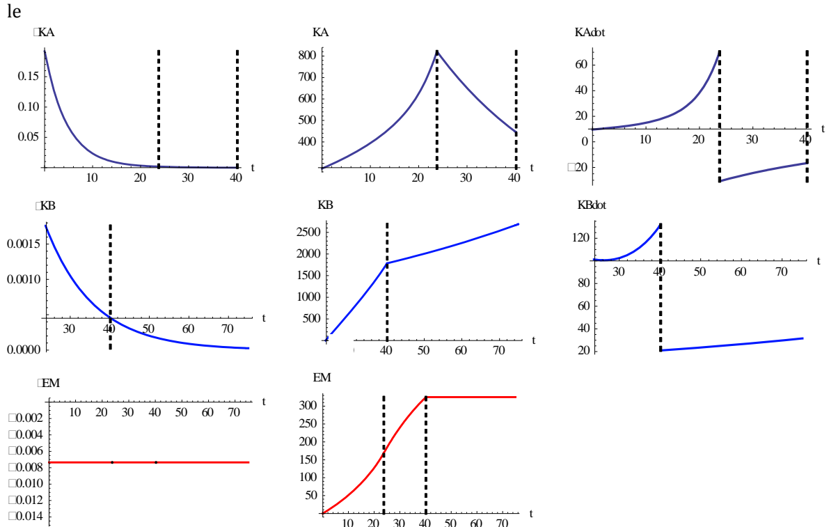
Figure 2.1 BAM baseline results for K_A , K_B and E
