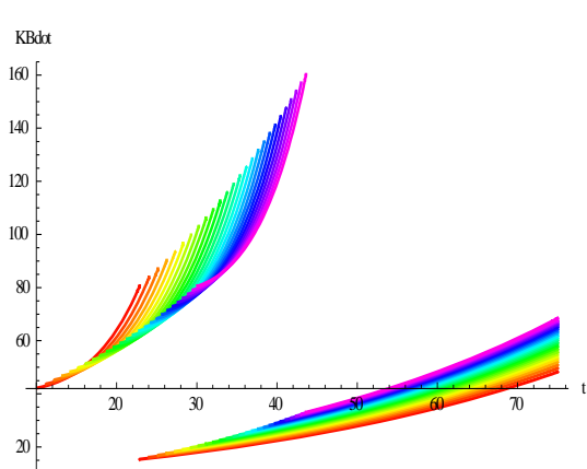
Figure 5.2.C capital K_B : Emax=125-375
