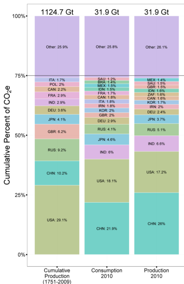
1 2 Figure SPM.4. Shares of largest country contributors to 75% of global anthropogenic CO 2 emissions 3 from fossil fuel combustion. Stacked bar on the left shows cumulative territorial emissions for the 4 period 1751-2009, stacked bar in the middle shows consumption based emissions in 2010 and the 5 stacked bar on the right shows production/territorial based emissions in 2010. [Figure 1.7]
