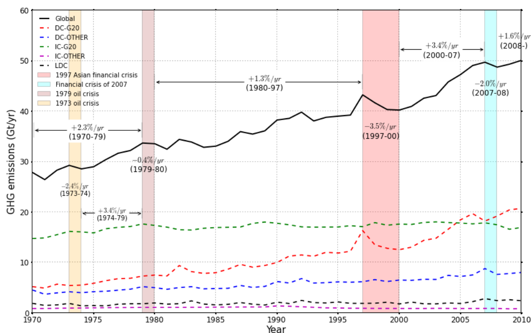
1 Figure SPM.1. Change in global anthropogenic GHG emissions by major economic regions 1970- 2 2010. GHG emissions are measured in gigatonnes per year (Gt/yr) of CO 2 equivalent. Non CO 2 3 greenhouse gases are converted to CO 2 equivalents using 100-year global warming potentials. Trend 4 lines show emission of industrialised countries with G20 membership (IC-G20, green), other 5 industrialised countries (IC-other, purple), developing countries with G20 membership (DC-G20, red), 6 least developed countries (LDC, dashed black), other developing countries (DC-other, blue). Global 7 emission trends (Global) are shown by the solid black line. Coloured areas identify periods of major 8 global economic recessions. [Figure 1.4]
