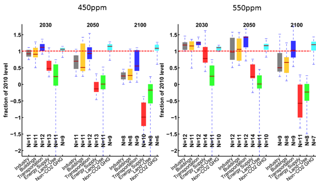
6 7 Figure SPM.11. Direct CO 2 emissions across sectors. The solid red lines correspond to the median, 8 the coloured box to the inter-quartile range (25th to 75th percentile) and the whiskers to the total 9 range across all reviewed scenarios. Dotted red line indicates relative emission level in 2010. [Figure 10 6.35]
