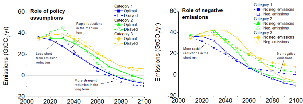
16 17 Figure SPM.6. Mean CO 2 emission pathways for different scenario categories according to 18 atmospheric CO 2 concentration stabilization levels in 2100: Category 1 (blue, 375-420 ppm CO 2 ), 19 Category 2 (green, 400-450 ppm CO 2 ), Category 3 (yellow, 450-495 ppm CO 2 ). The left panel 20 distinguishes between optimal and delayed policy responses, while the right panel indicates whether 21 a scenario includes negative emissions. [Figure 6.7]
