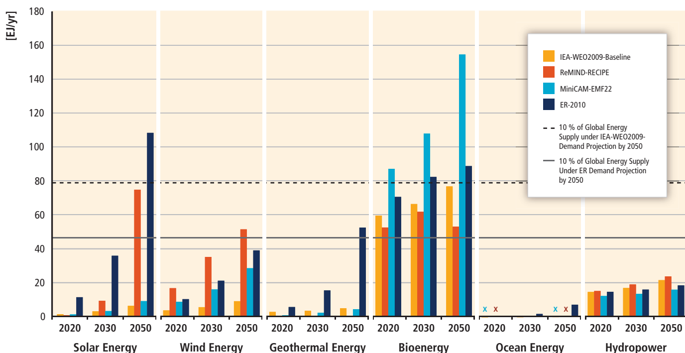
Figure TS.10.8 | Global RE development projections by source and global primary RE shares by source for a set of four illustrative scenarios. [Figure 10.14]
