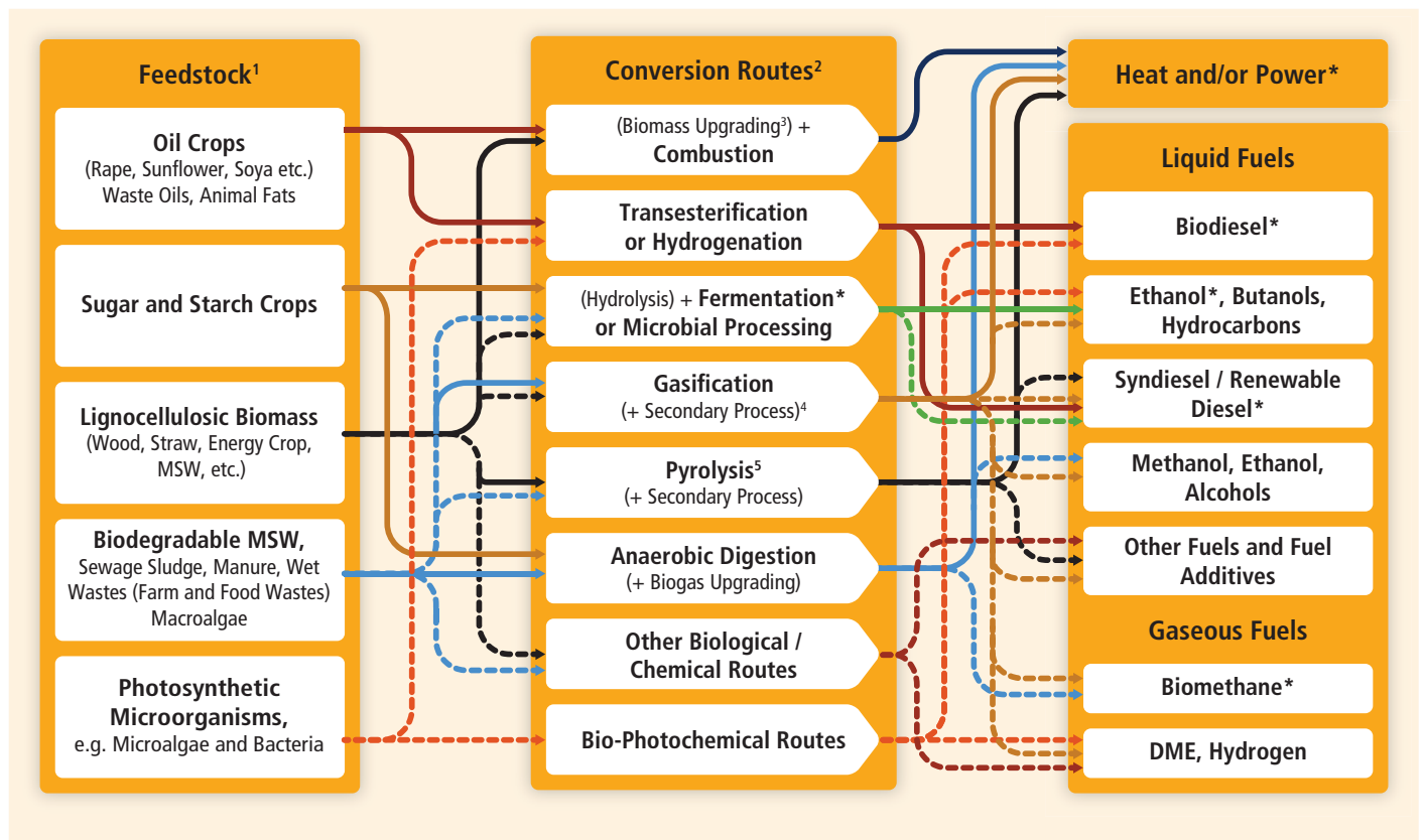
Figure TS.2.3 | Schematic view of the variety of commercial (solid lines) and developing bioenergy routes (dotted lines) from biomass feedstocks through thermochemical, chemical, biochemical and biological conversion routes to heat, power, CHP and liquid or gaseous fuels. Commercial products are marked with an asterisk. [Figure 2.2, 2.1.1]
