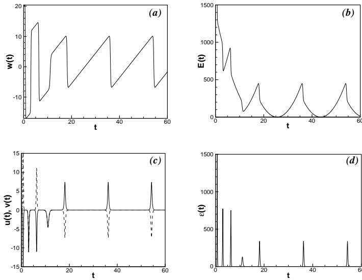
FIGURE 3. As in Figure 2 but for forced system (2.12, 2.13, 2.23).
