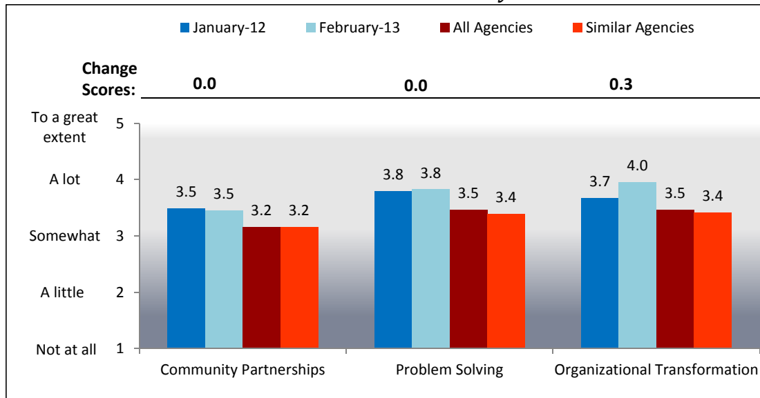
Exhibit 2.0. CP-SAT Summary
