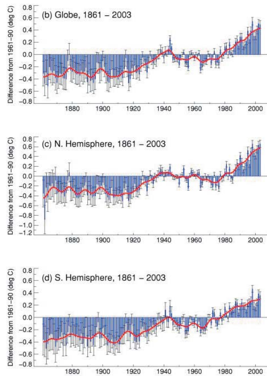
Figure 5. New global and hemispheric temperature series
