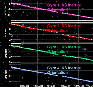
First results – Geodetic Precession
