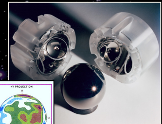
Gyroscope and housing
