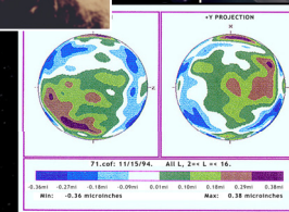
Rotor topology
