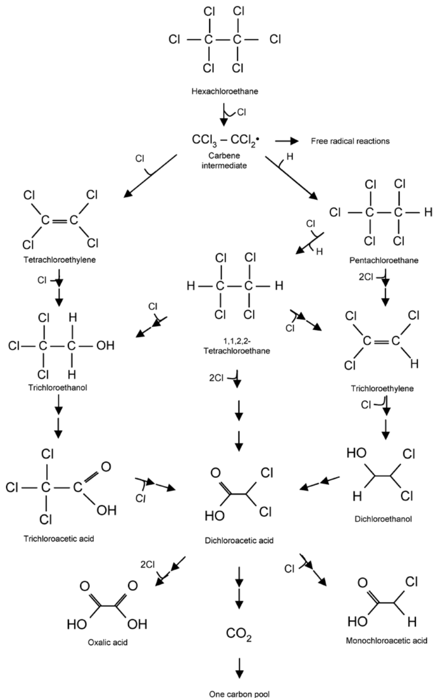
Figure 3-1 Plausible metabolic pathway of HCE
