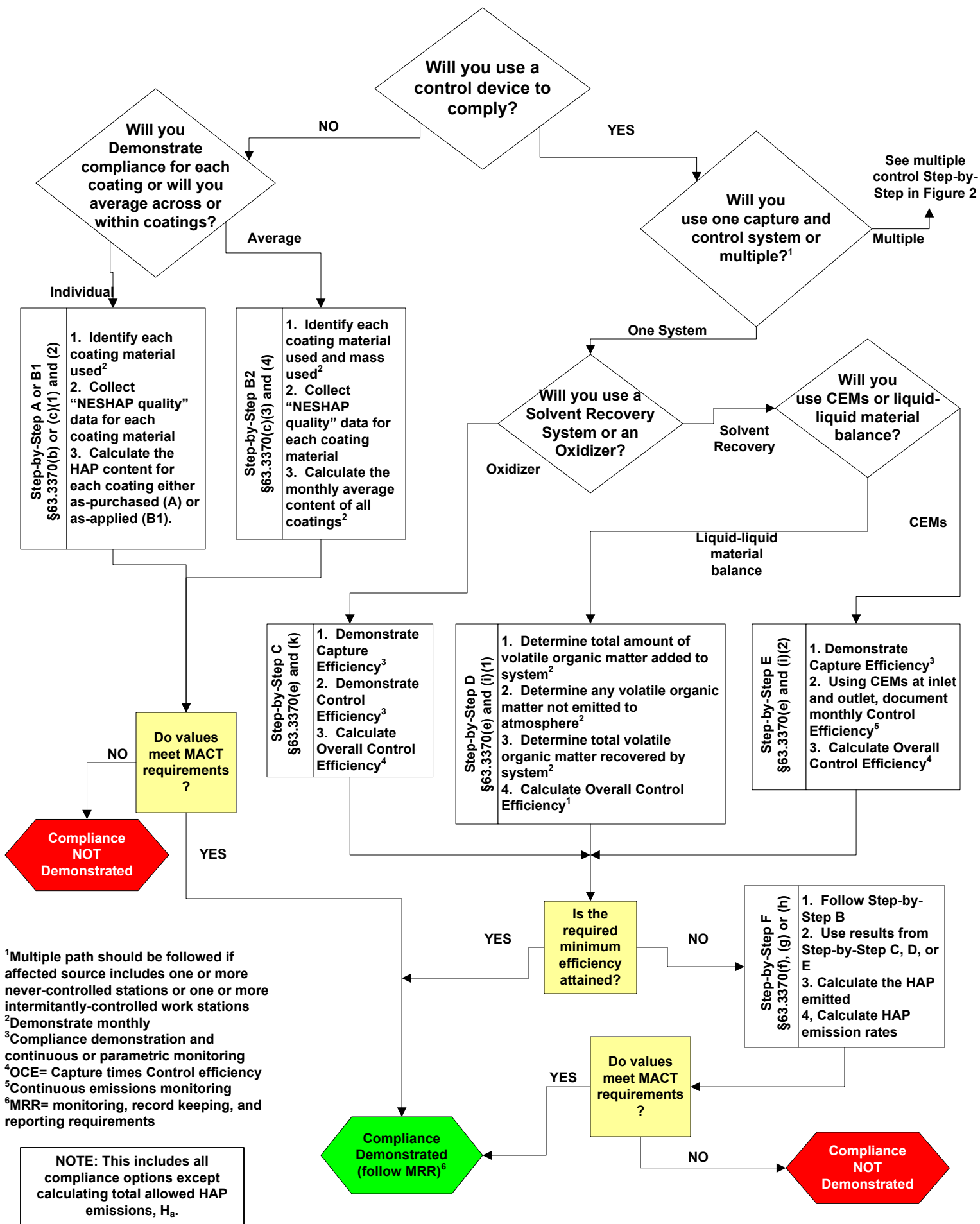
Figure 1. Compliance Alternatives for the Paper and Other Web MACT [40 CFR, Part 63, Subpart JJJJ]
