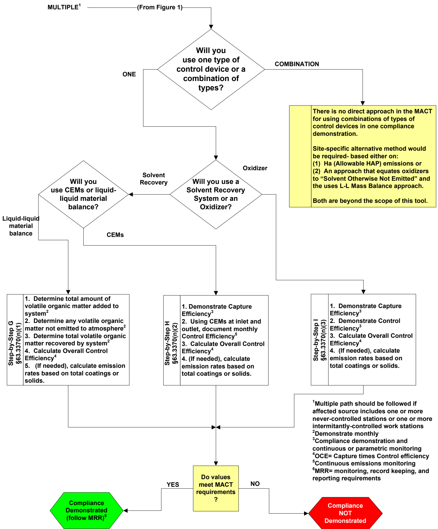
Figure 2. Compliance Alternatives for the Paper and Other Web MACT- Using Multiple Control Devices and/or Capture Systems [40 CFR, Part 63, Subpart JJJJ]
